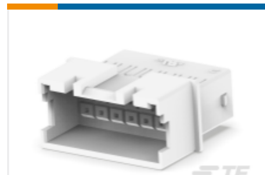
TE Part # 1-2324582-4 HSG,REC,FREE-HANGING,DUALROW, EP2.5
